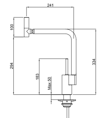
Schéma Technique Technical drawing
