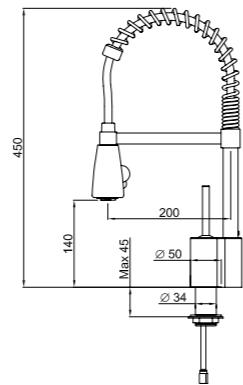
Schéma Technique Technical drawing
