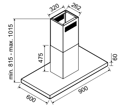
Schéma technique Technical drawing
