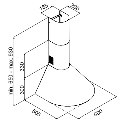
Schéma technique Technical drawing
