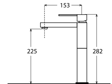
Schéma Technique Technical drawing
