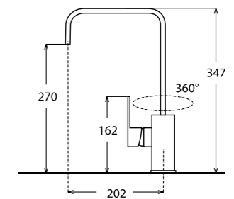
Schéma Technique Technical drawing
