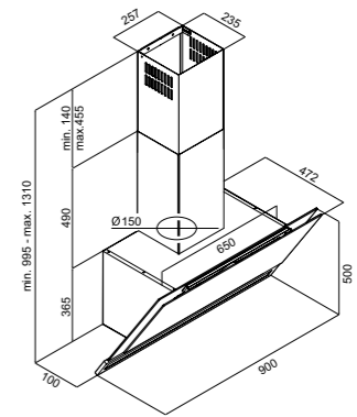
Schéma technique Technical drawing
